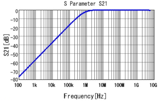
■ GCD188R71H222MA01 S21 DCOV, 25degC
