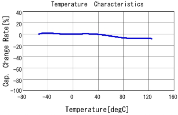
■ GCD188R71H222MA01 C-Temp. capchange, DCO. 0V, AC1. 0Vrm
