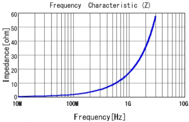
LQG15WH2N8B02 |Z|
