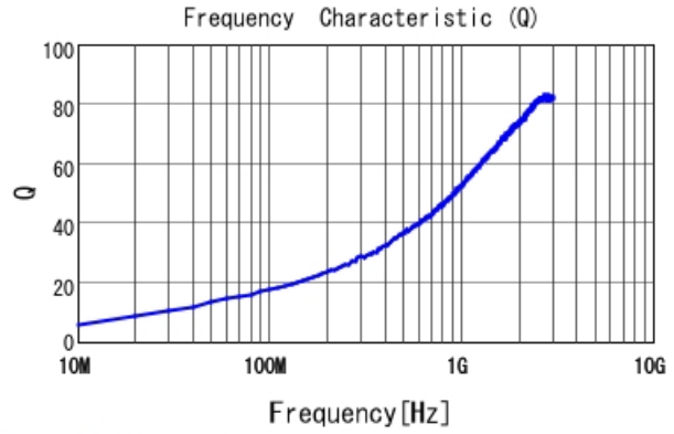
LQG15WH2N8B02 Q
