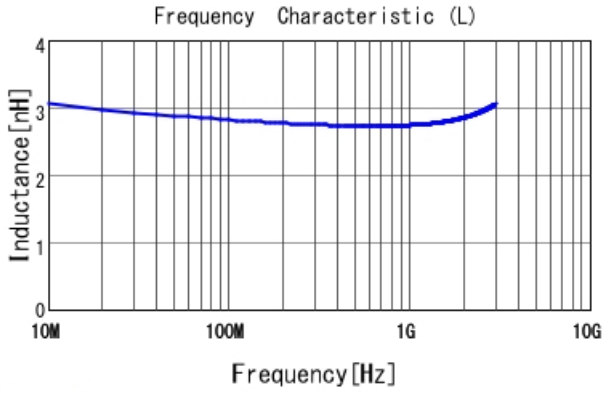
LQG15WH2N8B02 L
