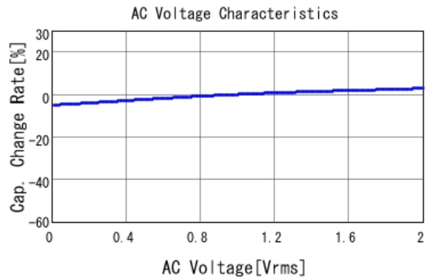
■ GCJ31CC71H475KA01 C-AC Voltage capchange, DC0V, 25.0d
