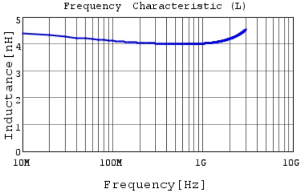
LQP03HQ4N0B02 L
