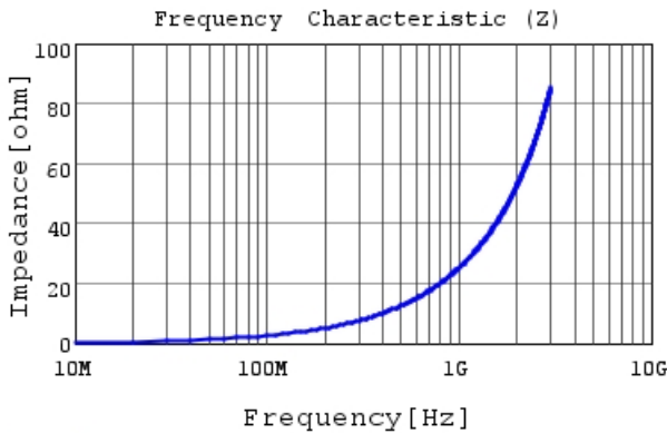
LQP03HQ4N0B02 |Z|
