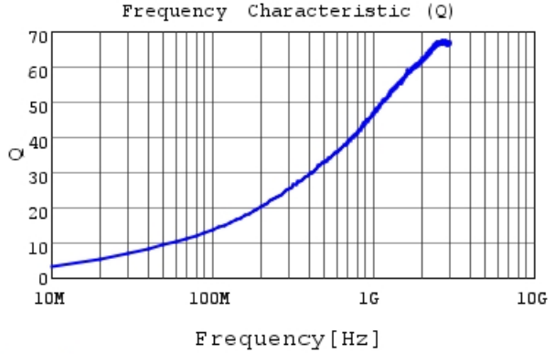
LQP03HQ4N0B02 Q
