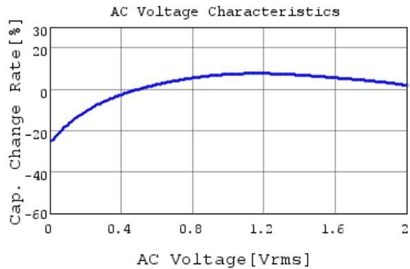
GRM188B30J106ME47 C-AC Voltage capchange, Dc
