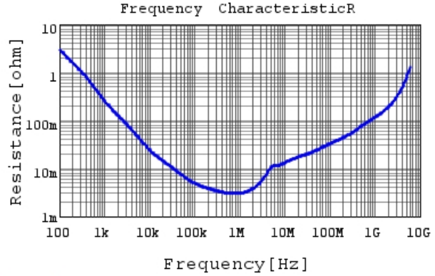
GRM188B30J106ME47 R DCOV, 20degC
