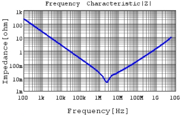
GRM188B30J106ME47 |Z| DCOV, 20degC
