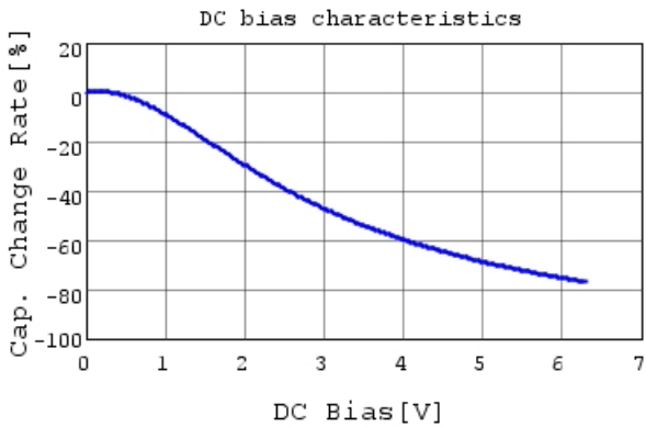
GRM188B30J106ME47 C-DC bias capchange, 20.0c
