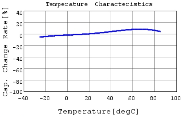
GRM188B30J106ME47 C-Temp. capchange, DC0.0V,
