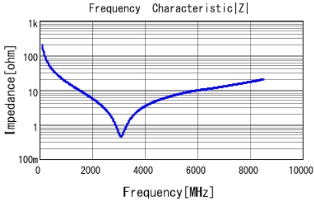
GRM1555C1H8R2WA01 |Z| DCOV, 25degC
