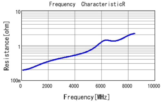
GRM1555C1H8R2WA01 R DCOV, 25degC
