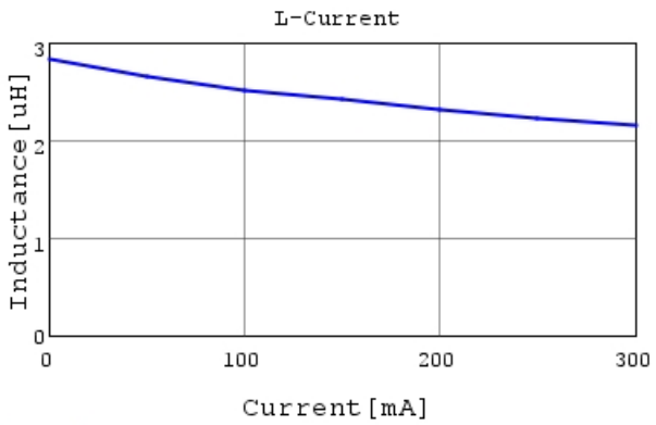
LQM21PN3R3NG0 L-Current 20degC
