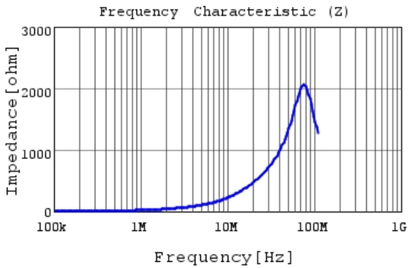
LQM21PN3R3NG0 |Z|
