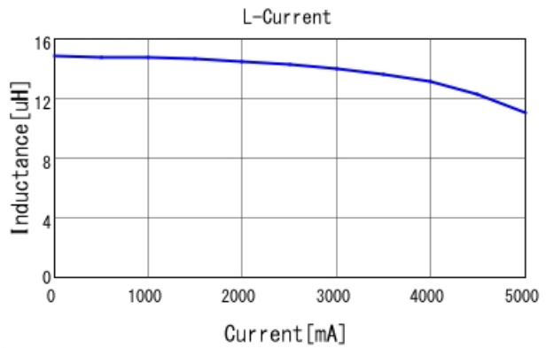
1217AS-H-150M L-Current 20degC
