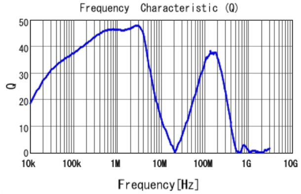
1217AS-H-150M Q
