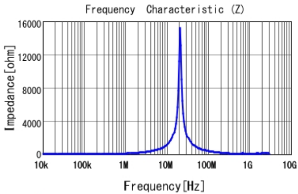
1217AS-H-150M |Z|
