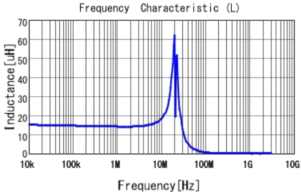
1217AS-H-150M L
