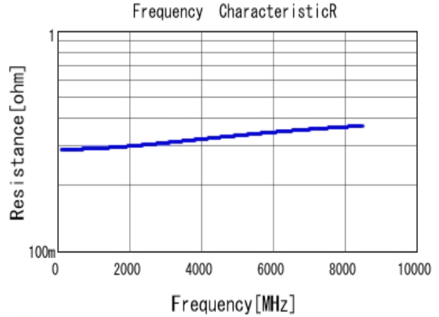
GJM0335C1E1R2WB01 R DC0V, 25degC
