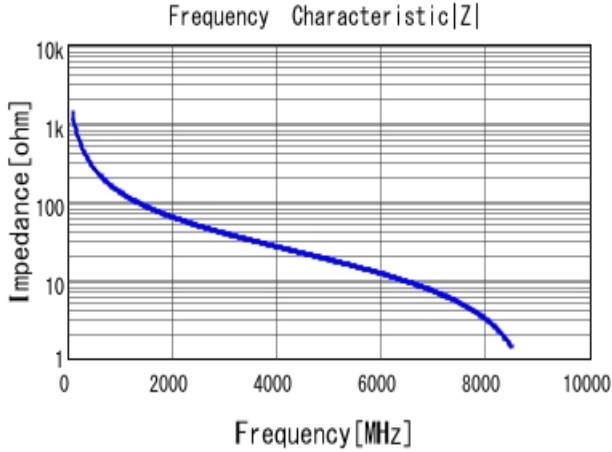
GJM0335C1E1R2WB01 |Z| DC0V, 25degC
