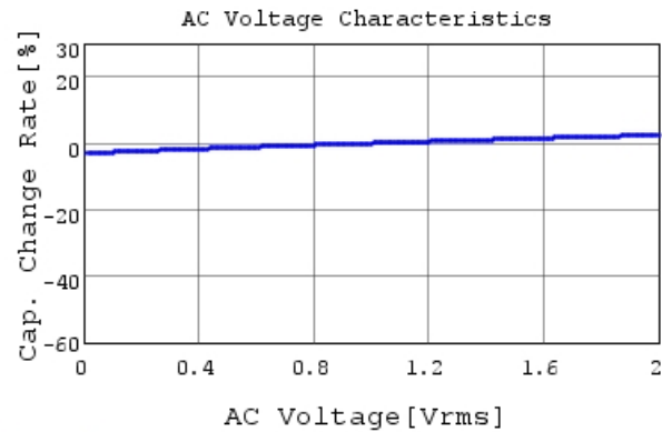
GCJ188R71H104KA12 C-AC Voltage capchange, Dc
