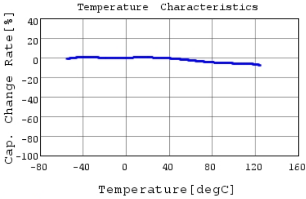
GCJ188R71H104KA12 C-Temp. capchange, DC0.0V,
