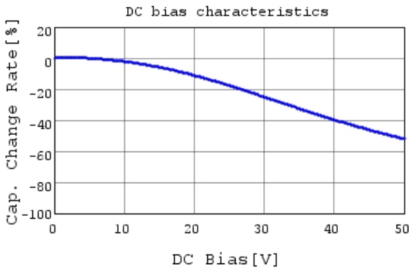
GCJ188R71H104KA12 C-DC bias capchange, 25.0c
