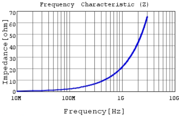
LQP02HQ3N4B02 |Z|
