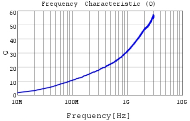
LQP02HQ3N4B02 Q
