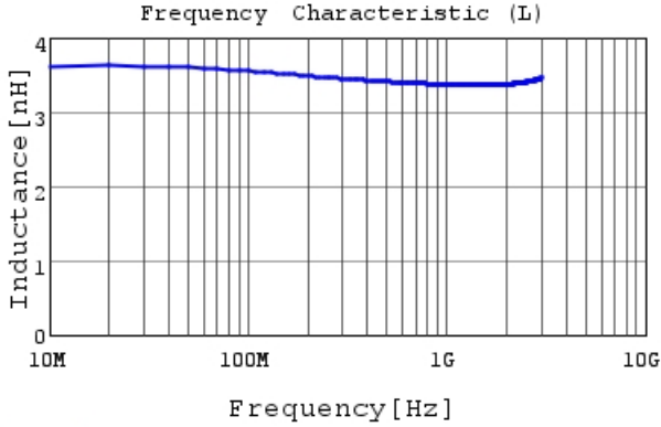
LQP02HQ3N4B02 L
