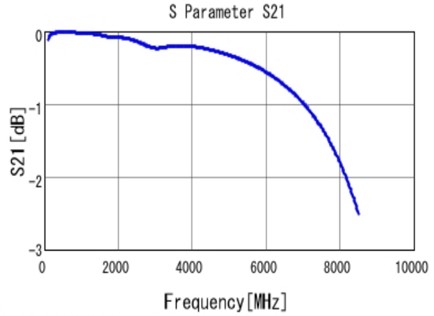
■ GRM1885C2A101JA01 S21 DCOV, 25degC
