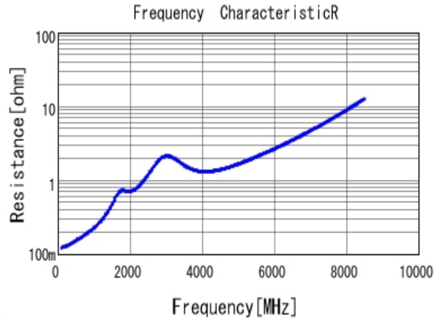
■ GRM1885C2A101JA01 R DCOV, 25degC
