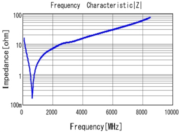
■ GRM1885C2A101JA01 |Z| DCOV, 25degC
