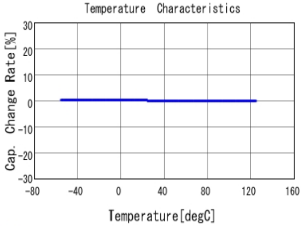
■ GRM1885C2A101JA01 C-Temp. capchange, DCOV, AC1Vrms
