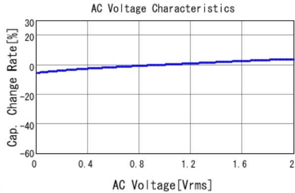
GRM155R11A473KA01 C-AC Voltage capchange, DCOV, 2C
