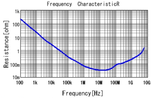
GRM155R11A473KA01 R DCOV, 20degC
