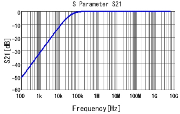
GRM155R11A473KA01 S21 DC0V, 20degC
