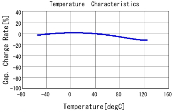
GRM155R11A473KA01 C-Temp. capchange, DC0.0V, AC1.C
