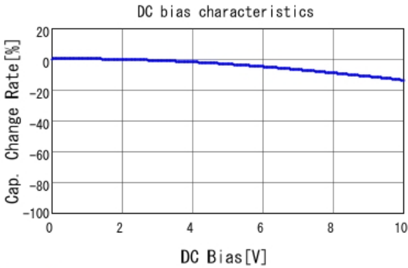
GRM155R11A473KA01 C-DC bias capchange, 20.0degC, A
