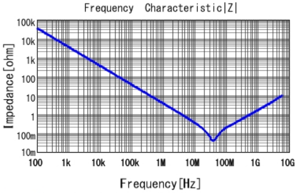
GRM155R11A473KA01 |Z| DCOV, 20degC
