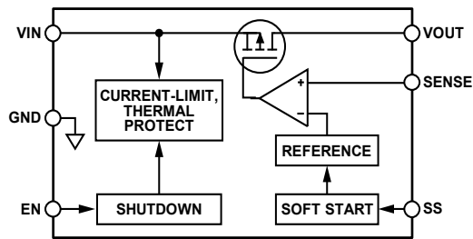
Figure 54. Internal Block Diagram
