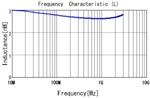
LQP03TN2N6C02 L
