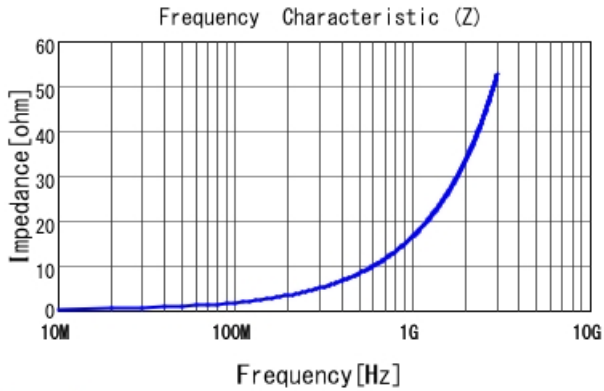
LQP03TN2N6C02 |Z|
