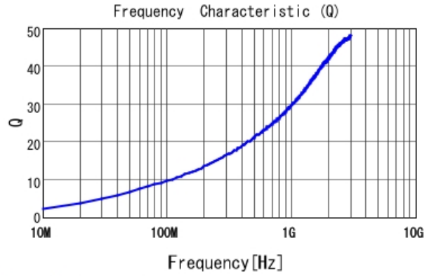
LQP03TN2N6C02 Q
