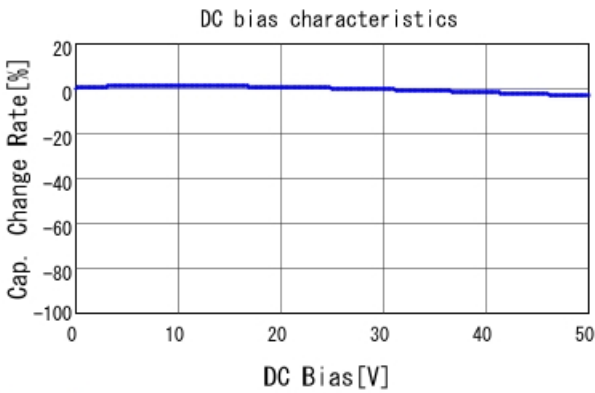
GRM188R71H471KA01 C-DC bias capchange, 25.0degC, A
