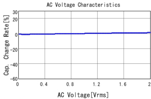
GRM188R71H471KA01 C-AC Voltage capchange, DCOV, 25
