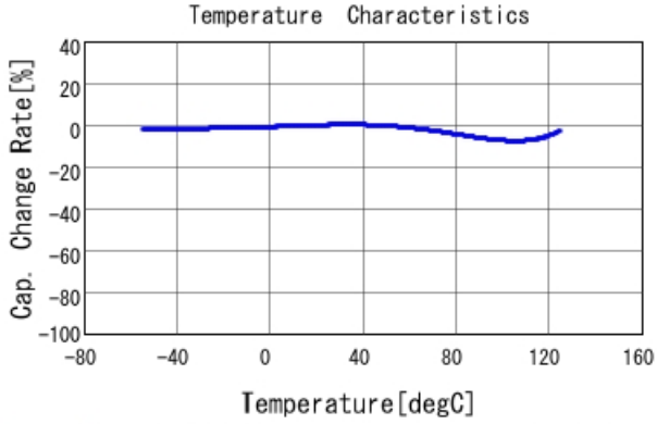
GRM188R71H471KA01 C-Temp. capchange, DC0.0V, AC1.C
