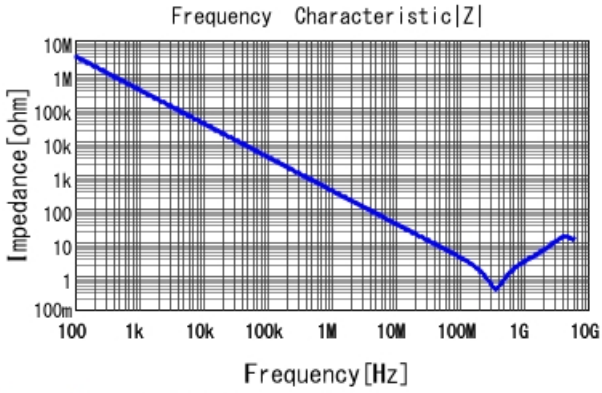
GRM188R71H471KA01 |Z| DCOV, 25degC
