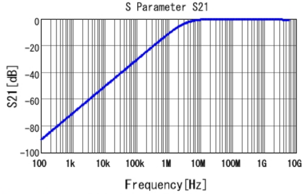
GRM188R71H471KA01 S21 DC0V, 25degC
