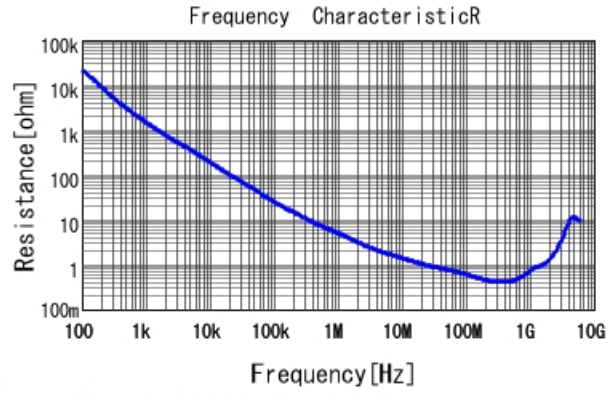
GRM188R71H471KA01 R DCOV, 25degC
