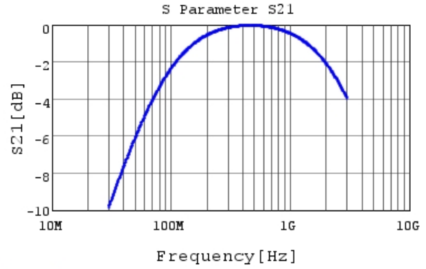
RDE5C1H180J0K1H03B S21 DCOV, 25degC
