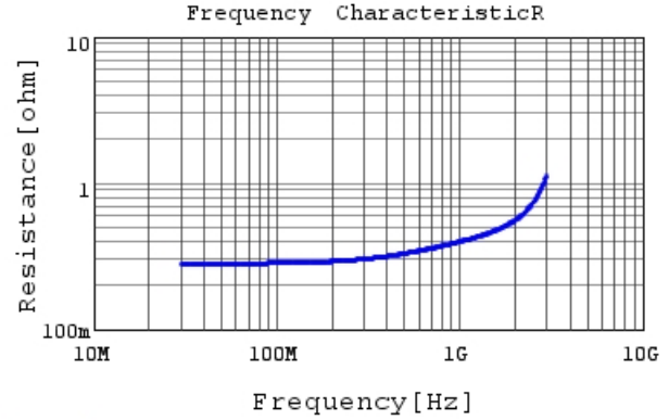
RDE5C1H180J0K1H03B R DCOV, 25degC
