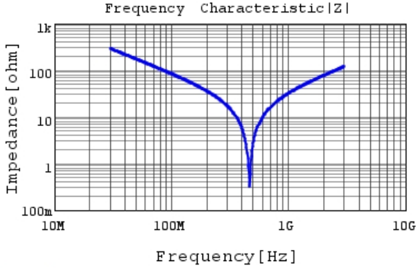
RDE5C1H180J0K1H03B |Z| DCOV, 25degC
