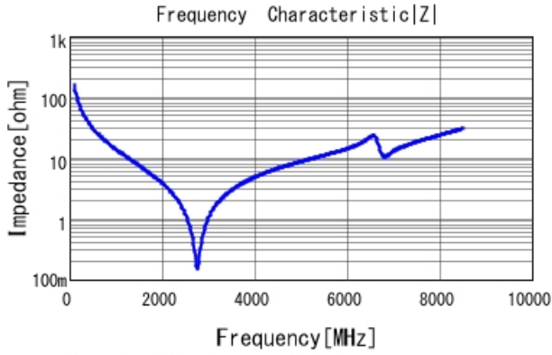
GJM1555C1H100GB01 |Z| DCOV, 25degC
