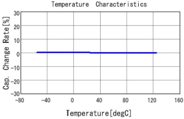
GRM0335C1E9R0DA01 C-Temp. capchange, DCOV, AC1Vrms
