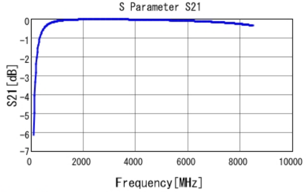
GRM0335C1E9R0DA01 S21 DCOV, 25degC
