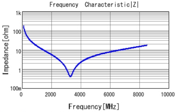
GRM0335C1E9R0DA01 |Z| DCOV, 25degC
