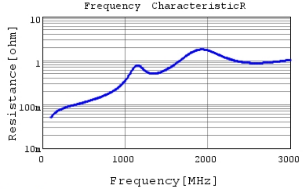
GRM21A5C2J221FWA1 R DC0V, 25degC
