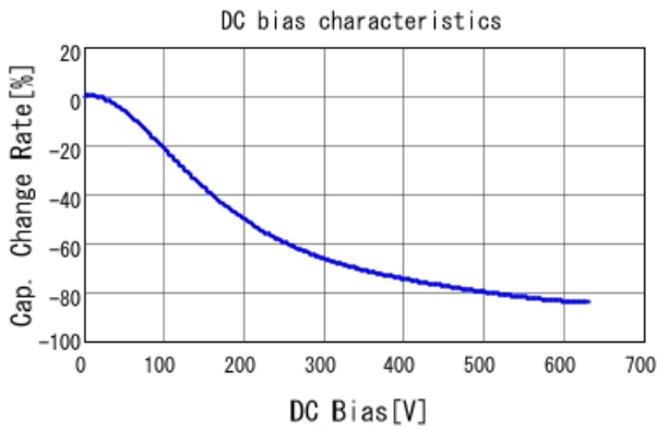
GRM31CR72J153KW03 C-DC bias capchange, 25.0degC, A
