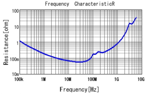
GRM31CR72J153KW03 R DCOV, 25degC
