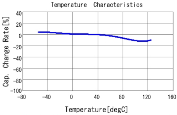
GRM31CR72J153KW03 C-Temp. capchange, DCOV, AC1Vrms
