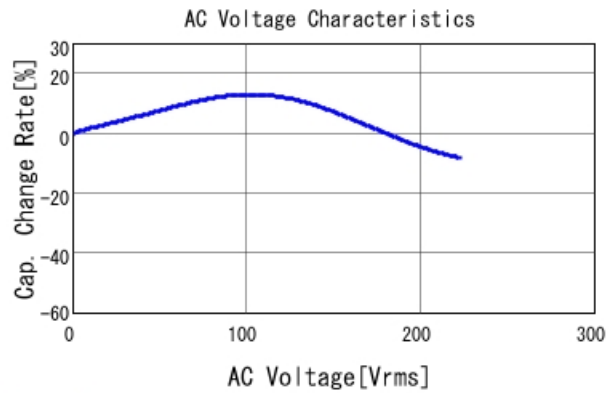
GRM31CR72J153KW03 C-AC Voltage capchange, DCOV, 25
