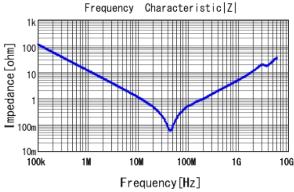
GRM31CR72J153KW03 |Z| DCOV, 25degC
