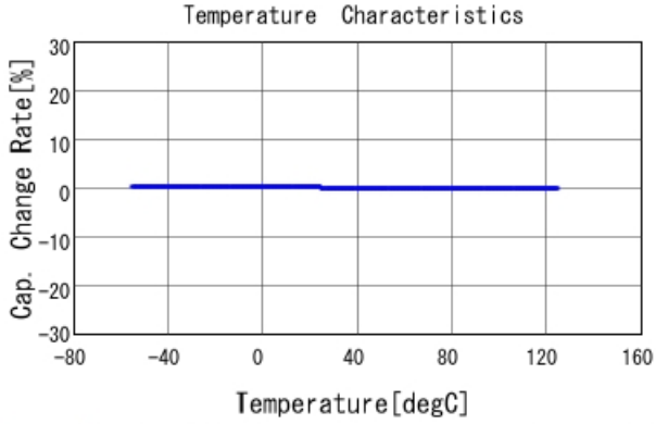
GRM1885C1H101JA01 C-Temp. capchange, DCOV, AC1Vrms
