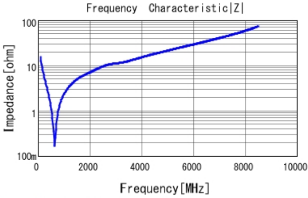
GRM1885C1H101JA01 |Z| DCOV, 25degC
