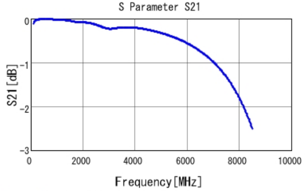
GRM1885C1H101JA01 S21 DCOV, 25degC
