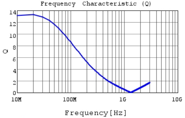
LQW18CNR27J00 Q
