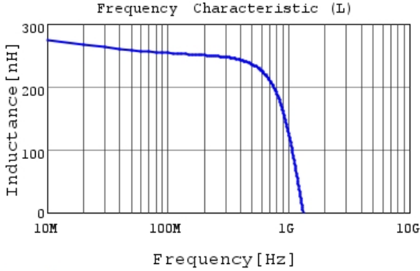
LQW18CNR27J00 L
