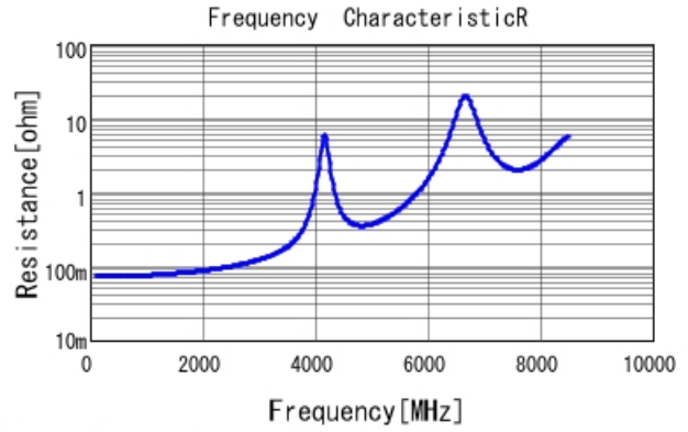
GJM1555C1H270FB01 R DCOV, 25degC
