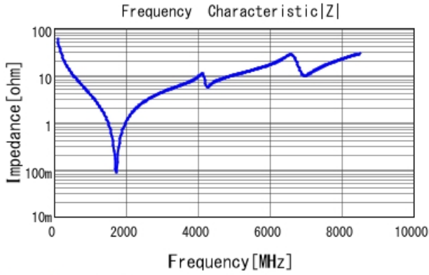
GJM1555C1H270FB01 |Z| DCOV, 25degC
