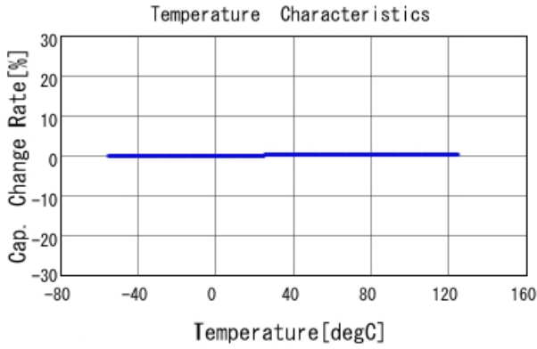
GJM1555C1H270FB01 C-Temp. capchange, DCOV, AC1Vrms
