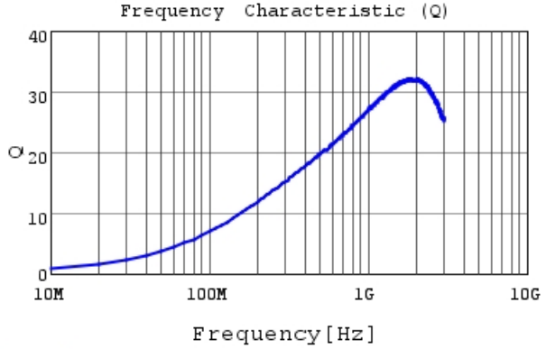
LQP15MN12NG02 Q
