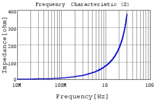
LQP15MN12NG02 |Z|
