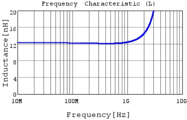
LQP15MN12NG02 L
