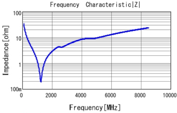
GRM1555C1E470JA01 |Z| DCOV, 25degC
