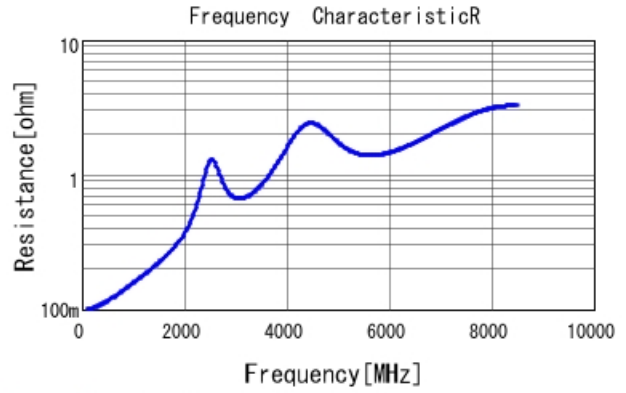
GRM1555C1E470JA01 R DCOV, 25degC
