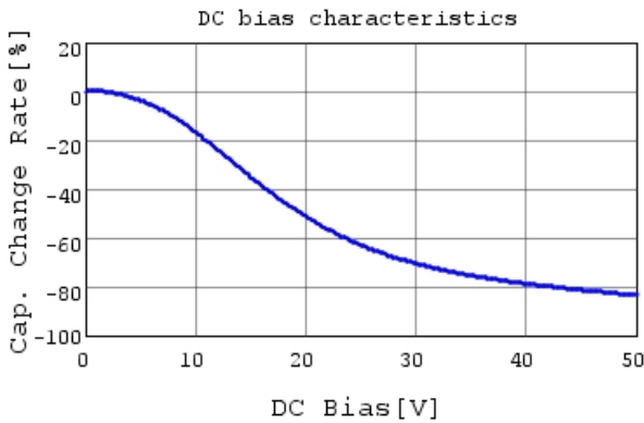
GRM155B31H104KE14 C-DC bias capchange, 20.0c
