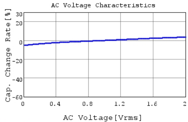
GRM155B31H104KE14 C-AC Voltage capchange, Dc
