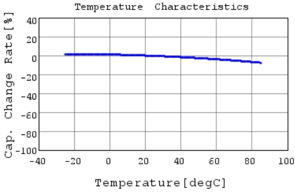
GRM155B31H104KE14 C-Temp. capchange, DC0.0V,
