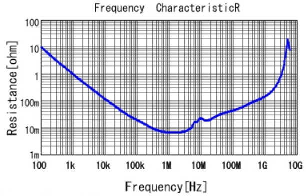
GRM319R61H475KA12 R DCOV, 25degC
