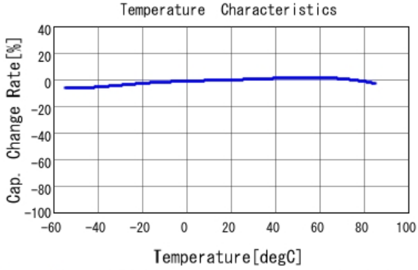
GRM319R61H475KA12 C-Temp. capchange, DC0.0V, AC1.C
