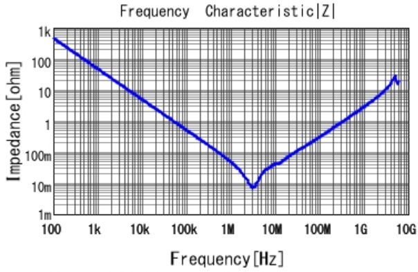
GRM319R61H475KA12 |Z| DCOV, 25degC
