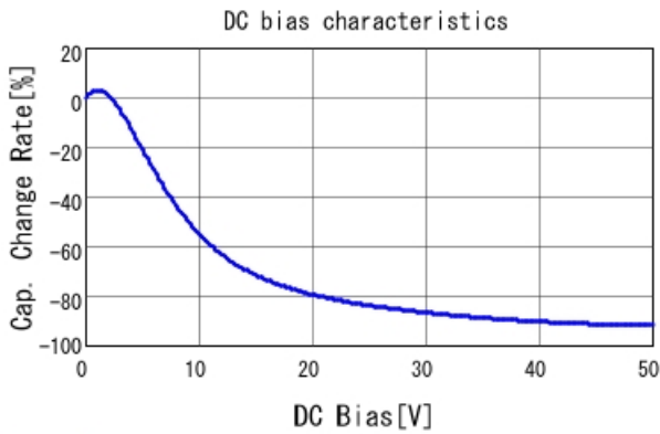
GRM319R61H475KA12 C-DC bias capchange, 25.0degC, A
