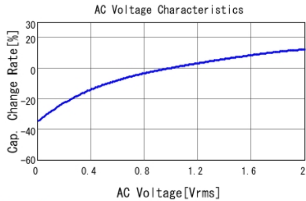
GRM319R61H475KA12 C-AC Voltage capchange, DCOV, 25
