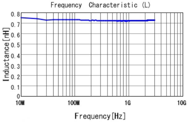
LQP03TN0N7B02 L
