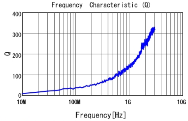
LQP03TN0N7B02 Q
