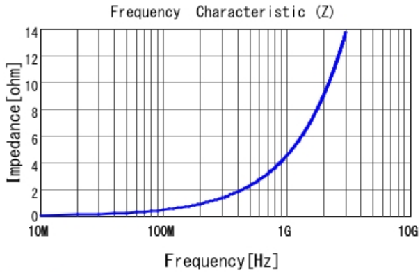
LQP03TN0N7B02 |Z|
