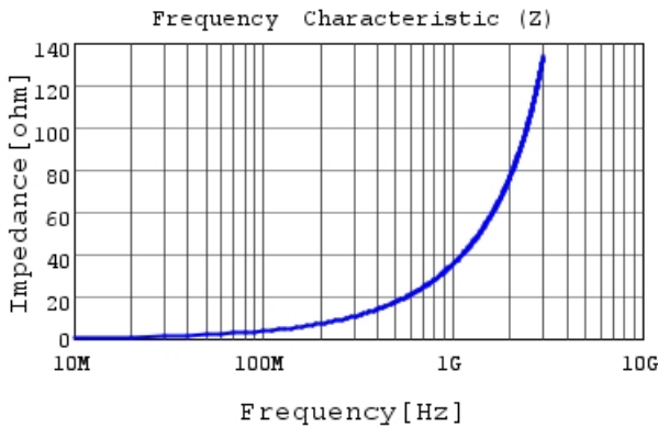
LQG15WZ5N6S02 |Z|
