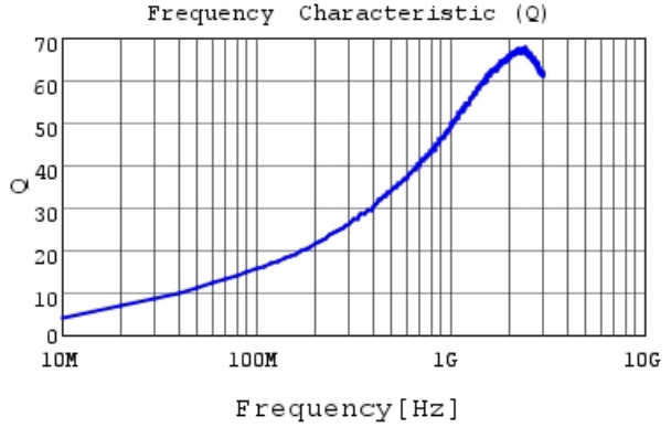
LQG15WZ5N6S02 Q
