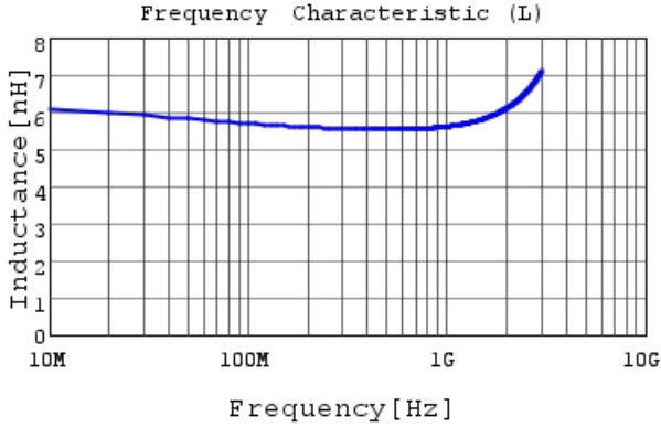
LQG15WZ5N6S02 L
