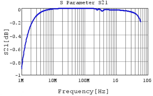
GCM1885C1H332JA16 S21 DCOV, 25degC
