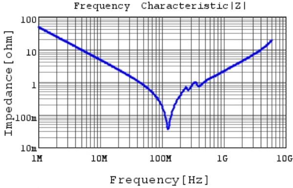
GCM1885C1H332JA16 |Z| DCOV, 25degC
