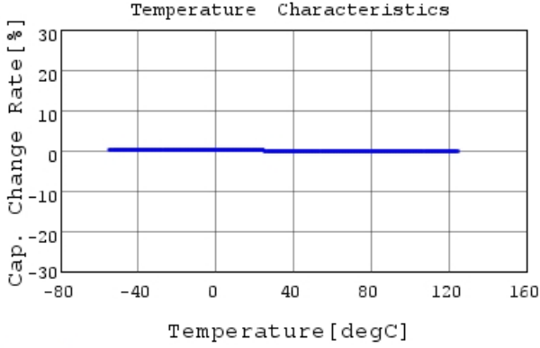
GCM1885C1H332JA16 C-Temp. capchange, DCOV, 1
