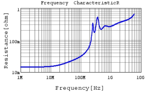
GCM1885C1H332JA16 R DCOV, 25degC
