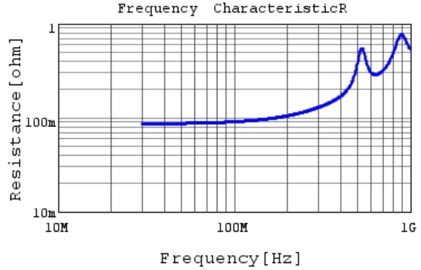
RCE5C2A681J0K1H03B R DCOV, 25degC
