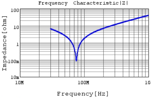
RCE5C2A681J0K1H03B |Z| DCOV, 25degC
