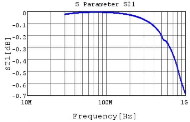
RCE5C2A681J0K1H03B S21 DCOV, 25degC
