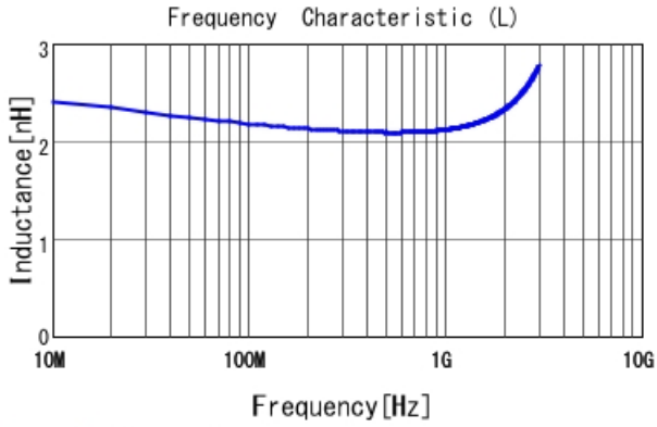
LQG15HH2N2C02 L
