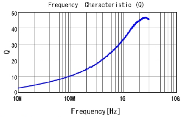
LQG15HH2N2C02 Q
