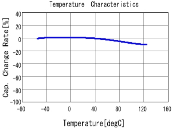
■ GRT31CR71H225KE13 C-Temp. capchange, DC0.0V, AC1.0V r m
