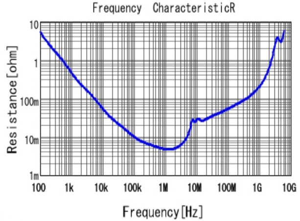
■ GRT31CR71H225KE13 R DCOV, 25degC
