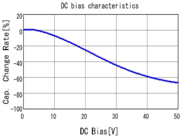
■ GRT31CR71H225KE13 C-DC bias capchange, 25.0degC, AC1.
