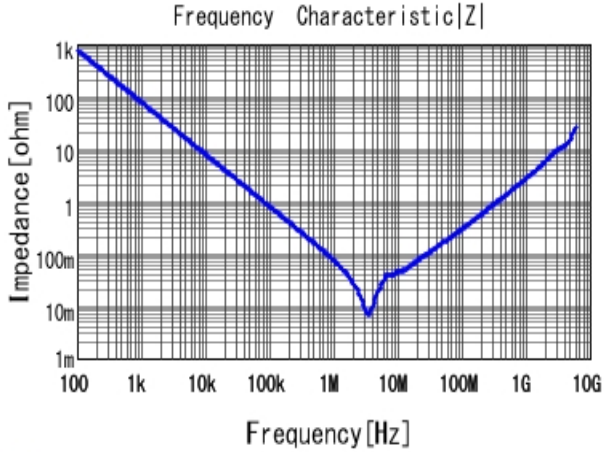
■ GRT31CR71H225KE13 |Z| DCOV, 25degC
