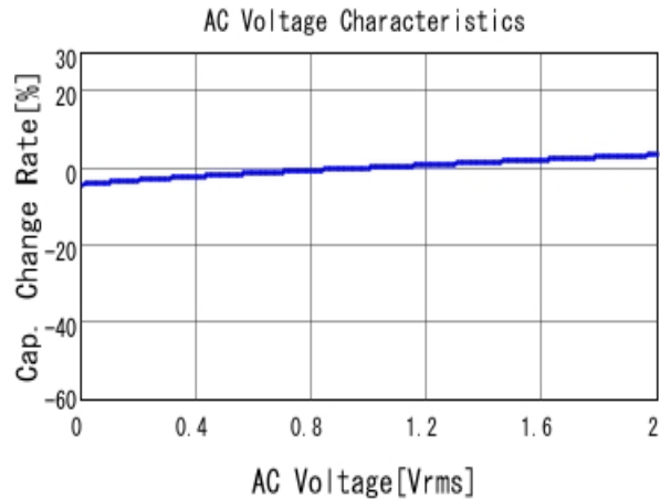
■ GRT31CR71H225KE13 C-AC Voltage capchange, DCOV, 25.0d
