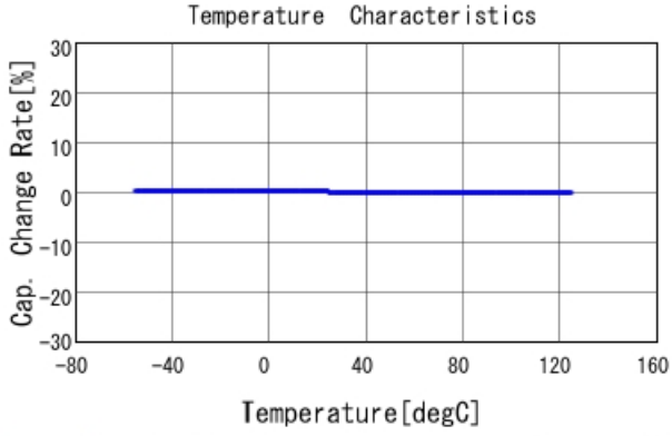
GRM1555C1H130JA01 C-Temp. capchange, DCOV, AC1Vrms
