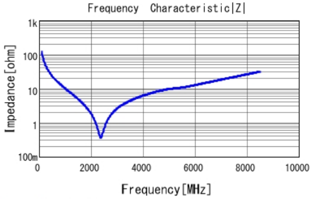
GRM1555C1H130JA01 |Z| DCOV, 25degC
