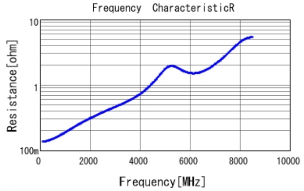
GRM1555C1H130JA01 R DCOV, 25degC
