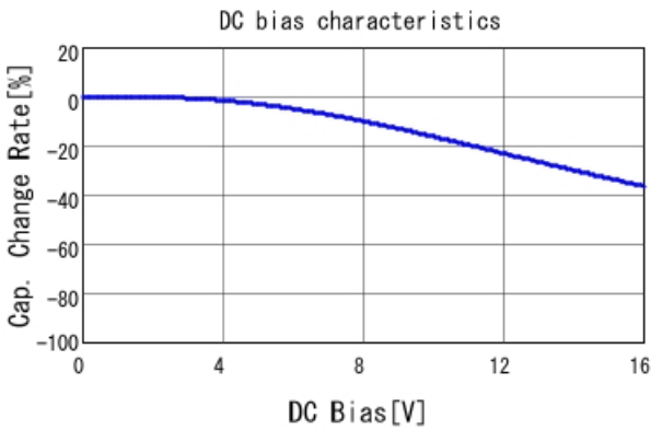
GRM21BR71C105KA01 C-DC bias capchange, 25.0degC, A
