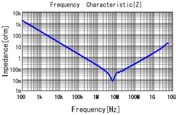
GRM21BR71C105KA01 |Z| DCOV, 25degC
