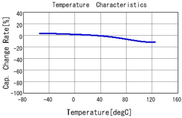
GRM21BR71C105KA01 C-Temp. capchange, DC0.0V, AC1.C
