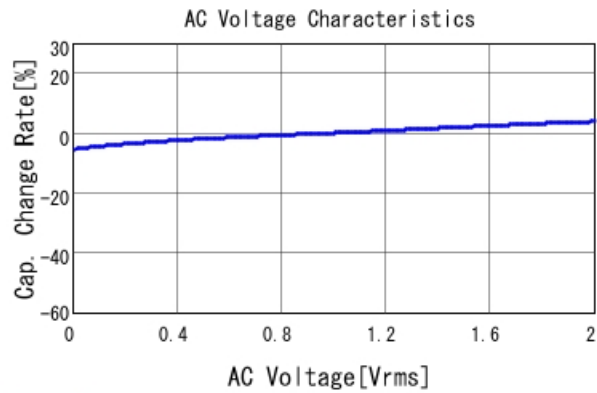
GRM21BR71C105KA01 C-AC Voltage capchange, DCOV, 25
