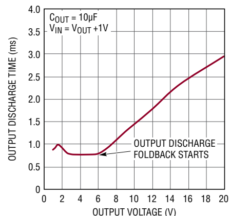
Figure 7. Discharge Time vs Output Voltage
