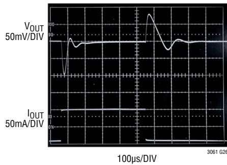
5V Transient Response C_{FF} = 0 , I_{OUT} = 10\text{mA} to 100\text{mA}
