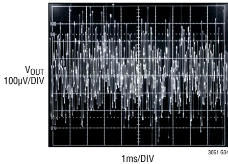
5V 10Hz to 100kHz Output Noise C_{REF/BYP} = 10\text{nF} , C_{FF} = 0
