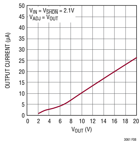
Figure 8. Reverse Output Current
