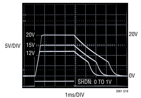
Output Discharge vs V_{OUT} C_{REF}/BYP = 0
