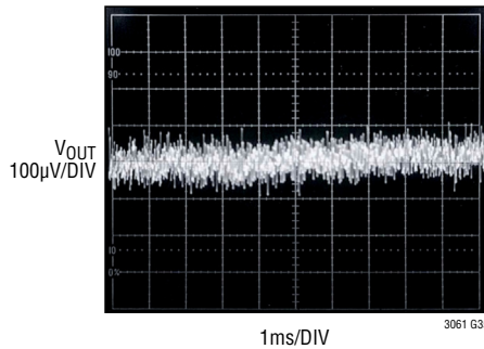
5V 10Hz to 100kHz Output Noise C_{REF/BYP} = 10\text{nF} , C_{FF} = 10\text{nF}
