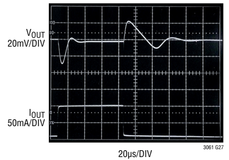
5V Transient Response C_{FF} = 10\text{nF} , I_{OUT} = 10\text{mA} to 100\text{mA}
