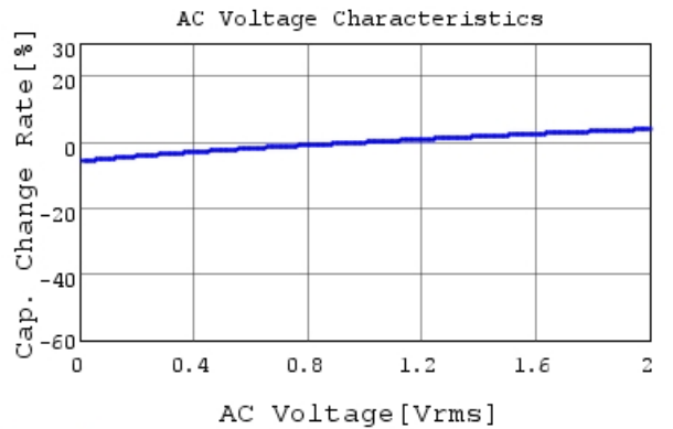
GRM31CC72A475ME11 C-AC Voltage capchange, Dc
