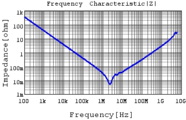
GRM31CC72A475ME11 |Z| DCOV, 25degC
