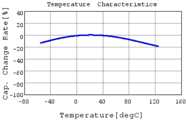
GRM31CC72A475ME11 C-Temp. capchange, DC0.0V,
