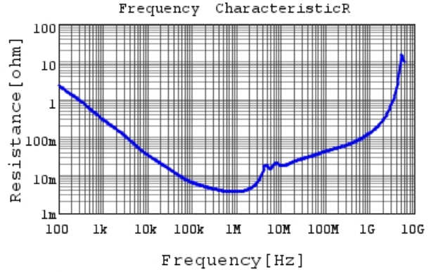
GRM31CC72A475ME11 R DCOV, 25degC
