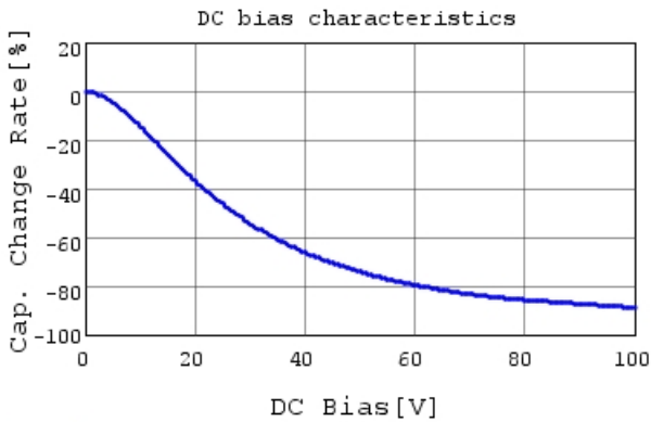
GRM31CC72A475ME11 C-DC bias capchange, 25.0c
