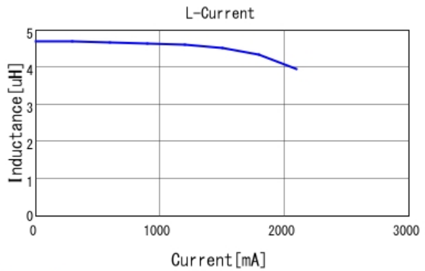
#A921CY-4R7M=P3 L-Current 20degC
