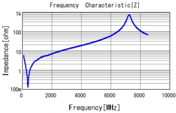
GCM1885C1H271JA16 |Z| DCOV, 25degC
