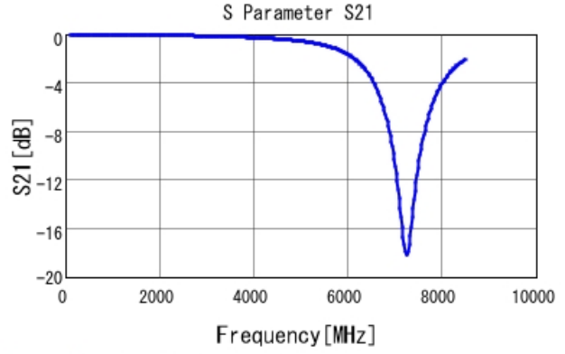
GCM1885C1H271JA16 S21 DCOV, 25degC
