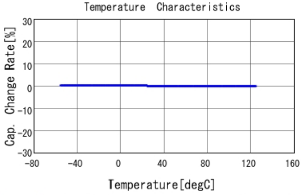
GCM1885C1H271JA16 C-Temp. capchange, DCOV, AC1Vrms
