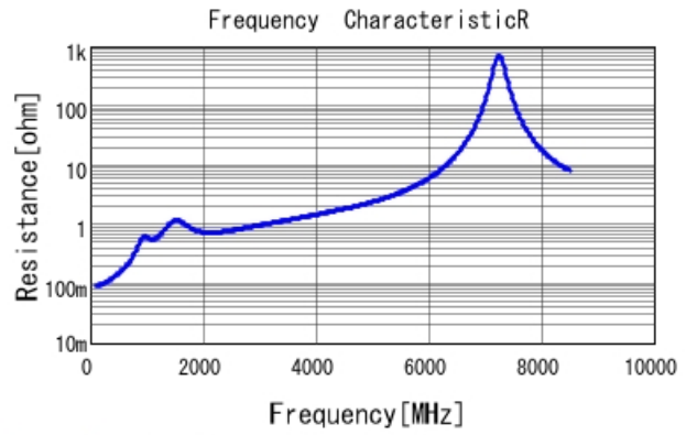
GCM1885C1H271JA16 R DCOV, 25degC
