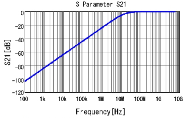
GRM033R61E101KA01 S21 DC0V, 25degC
