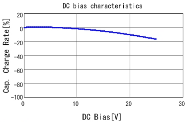
GRM033R61E101KA01 C-DC bias capchange, 25.0degC, A
