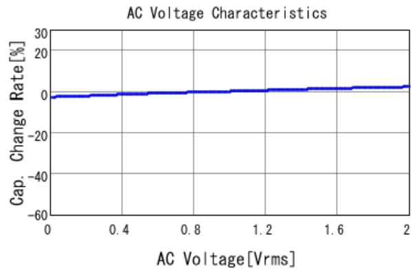
GRM033R61E101KA01 C-AC Voltage capchange, DCOV, 25
