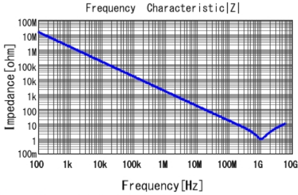
GRM033R61E101KA01 |Z| DCOV, 25degC
