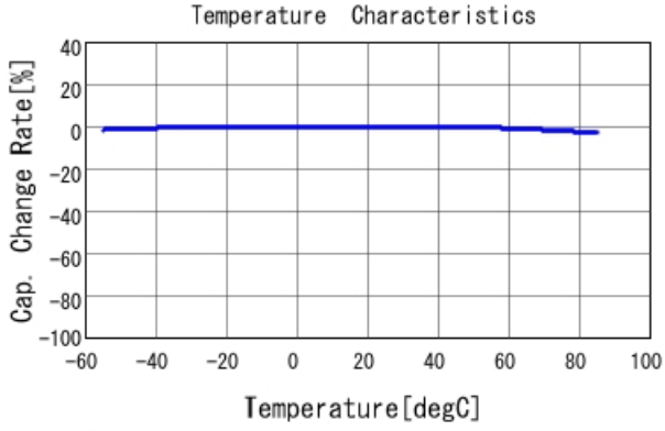
GRM033R61E101KA01 C-Temp. capchange, DC0.0V, AC1.C
