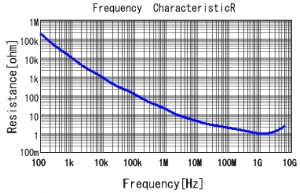
GRM033R61E101KA01 R DCOV, 25degC
