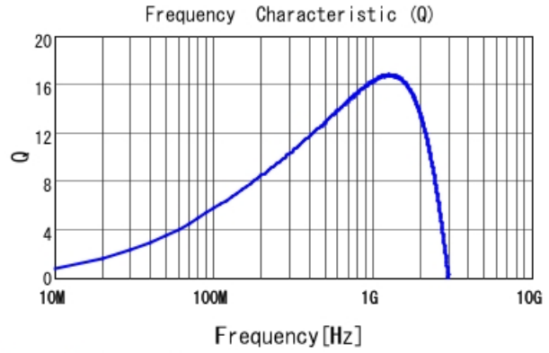
LQP03TG20NJ02 Q
