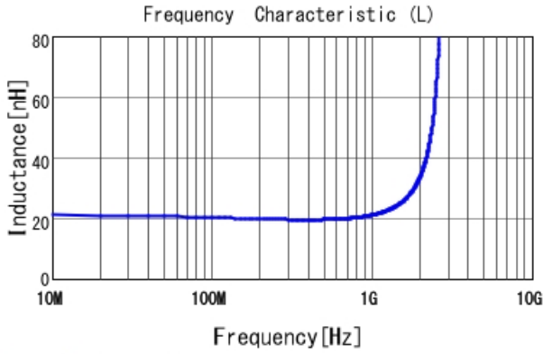
LQP03TG20NJ02 L
