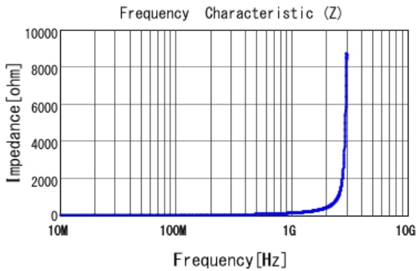
LQP03TG20NJ02 |Z|
