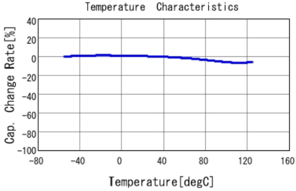
■ GRM033R71H471KA12 C-Temp. capchange, DCO. 0V, AC1. 0Vrm
