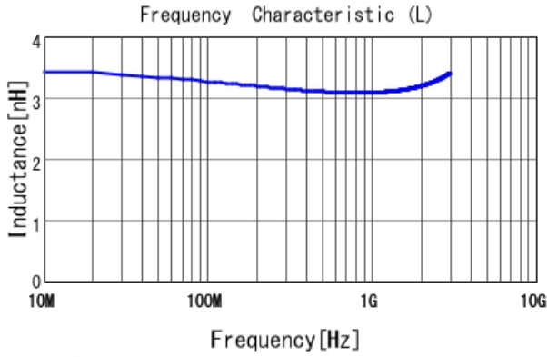
LQP03TG3N1B02 L
