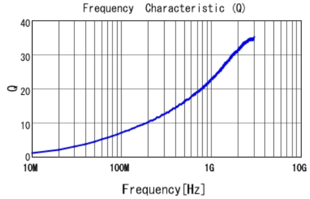
LQP03TG3N1B02 Q
