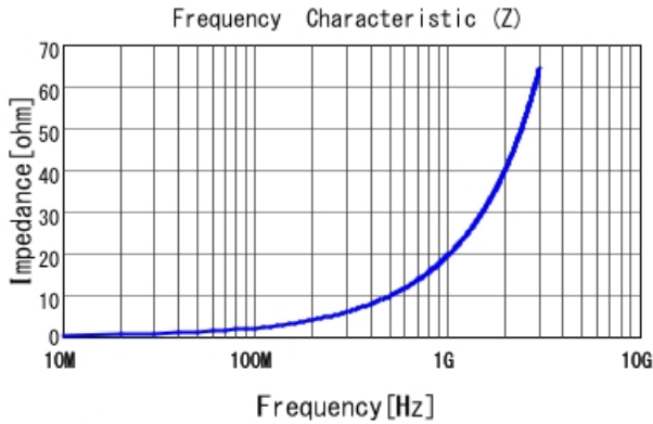
LQP03TG3N1B02 |Z|
