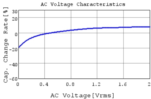
GRM155C70J225ME11 C-AC Voltage capchange, Dc
