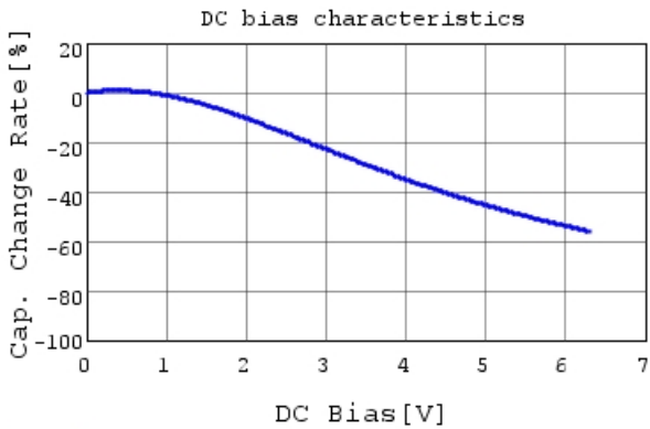
GRM155C70J225ME11 C-DC bias capchange, 25.0c
