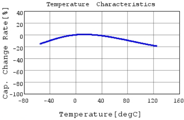
GRM155C70J225ME11 C-Temp. capchange, DC0.0V,
