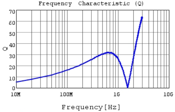
LQG18HN47NJ00 Q
