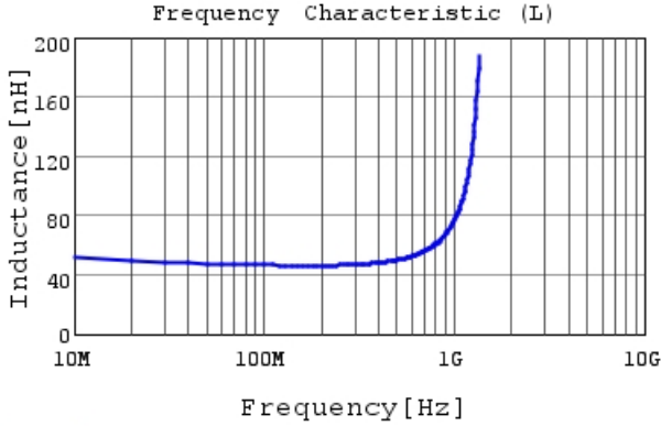
LQG18HN47NJ00 L
