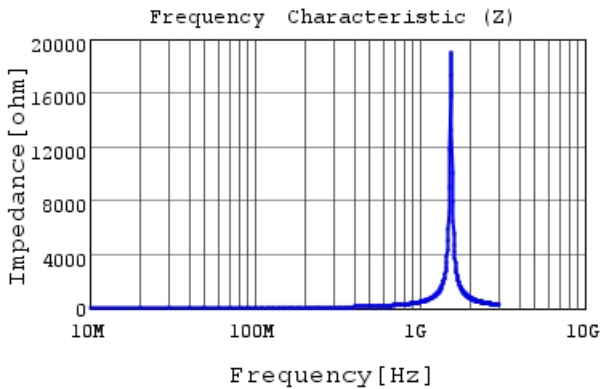
LQG18HN47NJ00 |Z|
