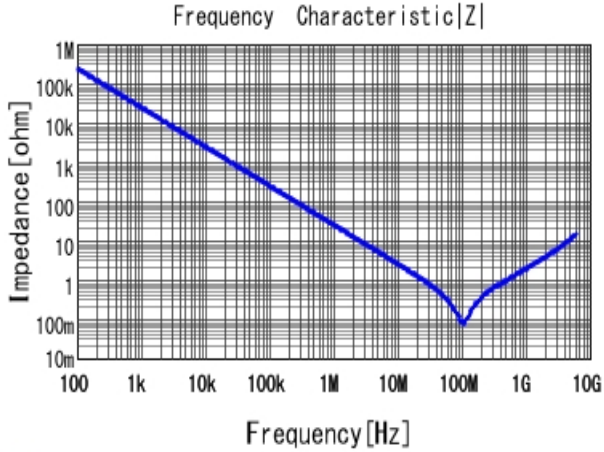
■ GRM155R71H682KA88 |Z| DCOV, 25degC
