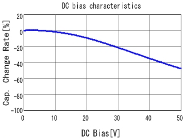
■ GRM155R71H682KA88 C-DC bias capchange, 25.0degC, AC1.
