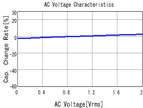
■ GRM155R71H682KA88 C-AC Voltage capchange, DCOV, 25.0d
