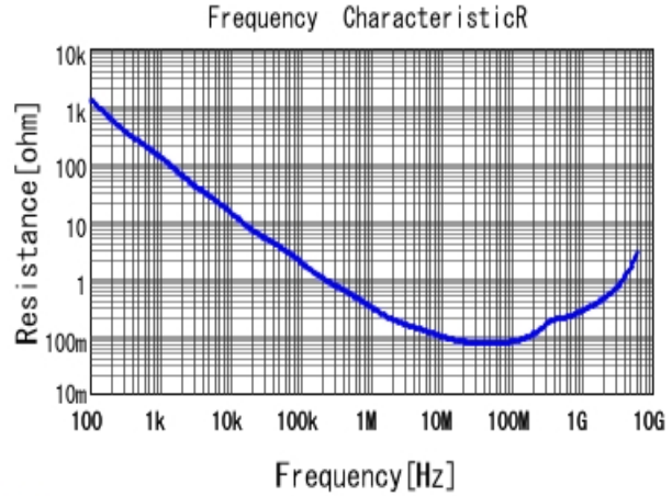
■ GRM155R71H682KA88 R DCOV, 25degC
