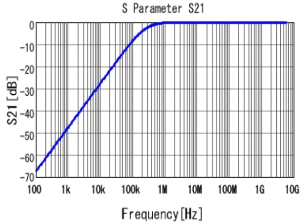
■ GRM155R71H682KA88 S21 DCOV, 25degC
