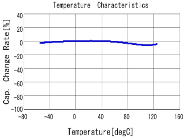
■ GRM155R71H682KA88 C-Temp. capchange, DCO. 0V, AC1.0Vrm
