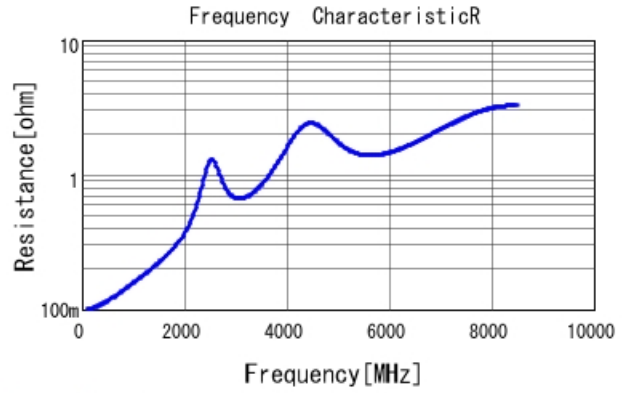
GRM1555C2A470JA01 R DCOV, 25degC
