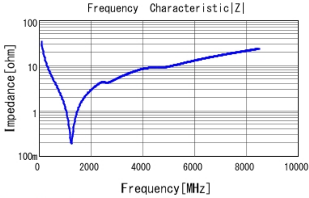
GRM1555C2A470JA01 |Z| DCOV, 25degC
