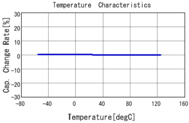
GRM1555C2A470JA01 C-Temp. capchange, DCOV, AC1Vrms
