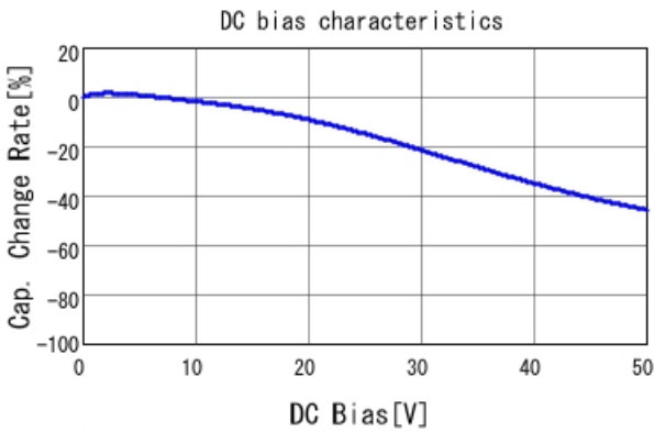
GRM155R61H222KA01 C-DC bias capchange, 25.0degC, A
