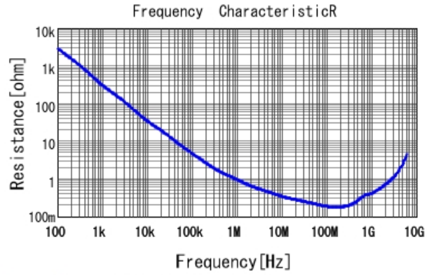
GRM155R61H222KA01 R DCOV, 25degC
