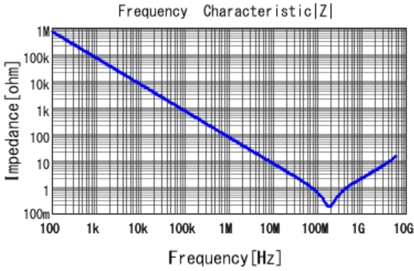
GRM155R61H222KA01 |Z| DCOV, 25degC
