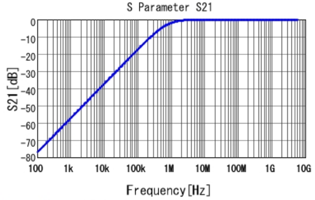
GRM155R61H222KA01 S21 DC0V, 25degC
