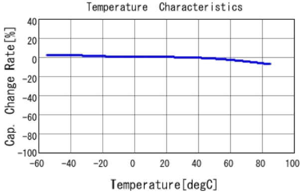
GRM155R61H222KA01 C-Temp. capchange, DC0.0V, AC1.C
