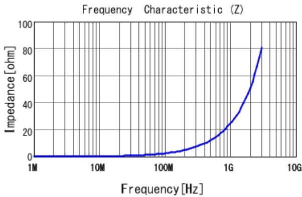
LQW15AN4N0G80 |Z|
