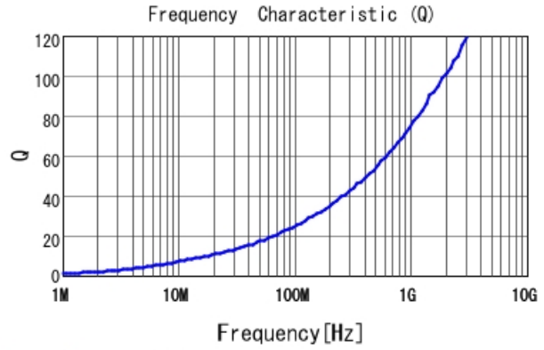
LQW15AN4N0G80 Q
