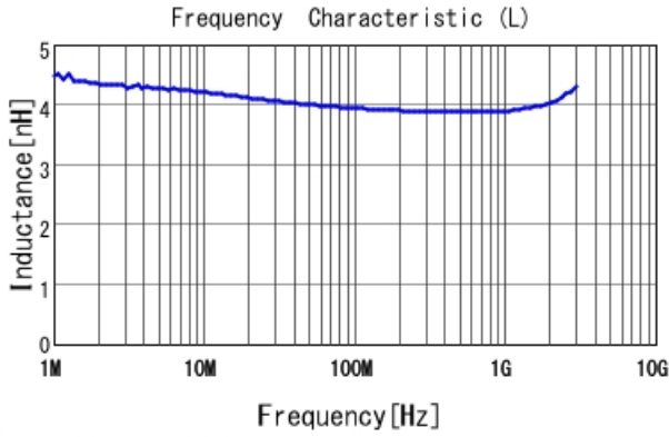
LQW15AN4N0G80 L
